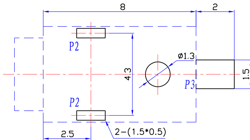
Dimensions of PC board holes (Commend)
